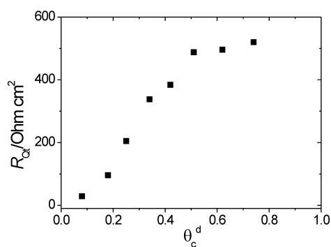
Figure 8. R_{Qr} versus \theta_c^d dependence extracted employing the model described in [24].
