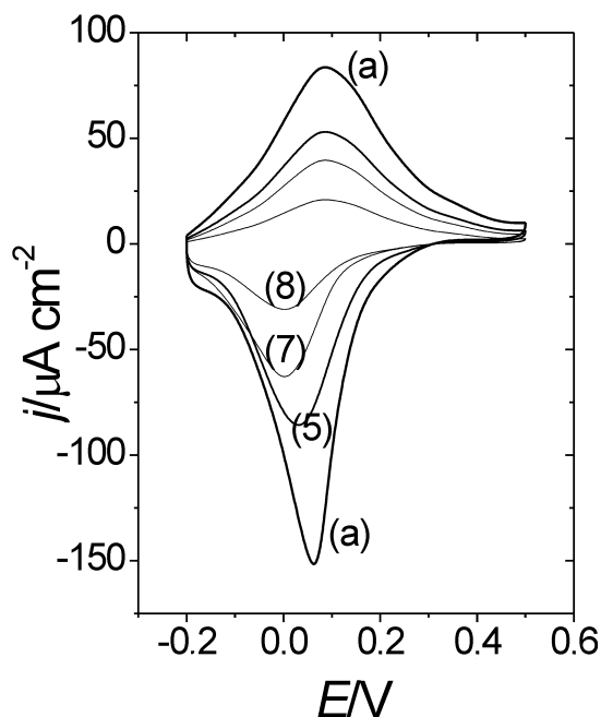
Figure 1. Voltammetric ( j - E ) responses for a 2.8 mC cm -2 ( \phi_p = 60 nm) thick POAP film. (a) A nondeactivated POAP film ( \theta_c^d = 0 ). Curves (5), (7) and (8) correspond to films whose degree of deactivation is: \theta_c^d = 0.42 ; \theta_c^d = 0.62 and \theta_c^d = 0.74 , respectively. Electrolyte: 0.1M HClO 4 + 0.4M NaClO 4 . Scan rate: \nu = 0.01 V s -1 .
