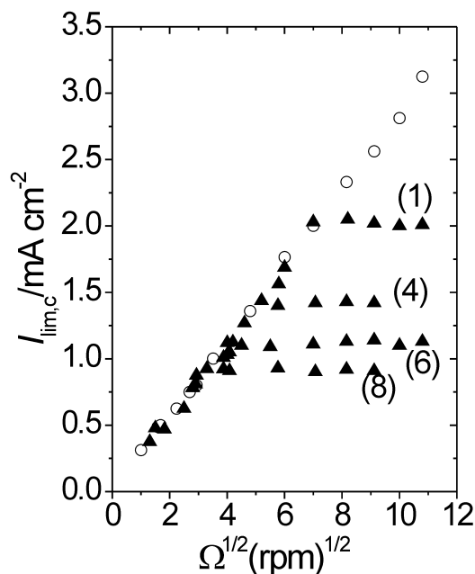
Figure 4. Levich representations I_{lim,c} versus \Omega^{1/2} for POAP films contacting a 0.1M \text{HClO}_4 + 0.4M \text{NaClO}_4 + 2 \times 10^{-3} M (HQ/Q) solution. (O) A nondeactivated POAP film. (1), (4), (6) and (8) correspond to the four films indicated in Table 1.
