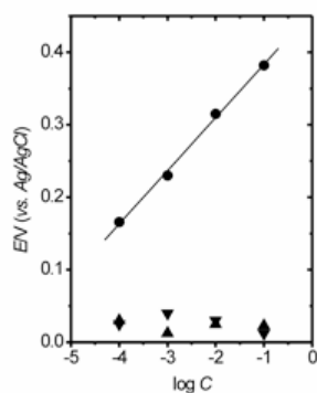
Figure 8. Relationship between the electrode potential, E, and the logarithm of the concentration, log C. (●) Fe (III); (▲) Ni(II), (▼) Zn(II) [36]. POAP films soaked for 24 h in a 0.1 \text{ M} H 2 SO 4 aqueous solution containing 50 \text{ mM} Fe 2 (SO 4 ) 3 [38].
