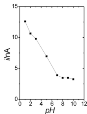
Figure 11. Amperometric currents developed by a POAP-modified electrode
