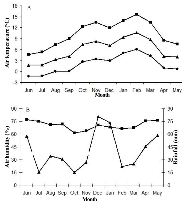
Figure 1. Climatic data for the experimental region near Ushuaia city, 54°48' SL, 68°19' WL (Tierra del Fuego, Argentina). A. Maximal (—■—), minimal (—◆—) and mean (—▲—) air daily temperatures, B. Mean ambient relative humidity (—■—) and rainfall (—▲—) were recorded from June 2010 to May 2011.
