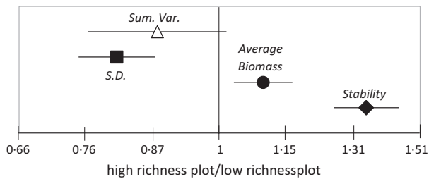
Fig. 3. The effect of species richness (SR) on stability and its different components, while holding PD (PD) constant. For the 1417 contrasts used in type 2 analysis, we further calculated the log ratios for community stability, average community biomass, standard deviation of biomass (SD) and sum of variances of individual species' biomass (sum.var.) in plots through time for higher vs. lower species richness. Positive log ratios for stability and biomass indicate that more speciose communities are more stable and produce more biomass than less speciose ones. Negative log ratios for SD indicate that the biomass of more speciose communities has lower temporal variation than the biomass of less speciose communities. Data points are the mean and 95% confidence intervals. Note that synchrony is not represented because it is not possible to estimate log ratios on negative values.
