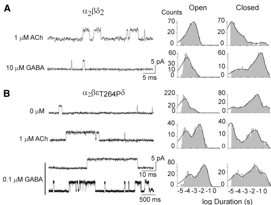
Fig. 3. (A) Activation of triplet \alpha_2\beta\delta_2 nAChRs. Single channels activated by 1 \mu\text{M} ACh and 10 \mu\text{M} GABA were recorded from cells expressing adult muscle nAChR lacking the \epsilon subunit. Left, traces of currents are shown at a bandwidth of 7 kHz with channel openings as upward deflections. Right, open and closed time histograms corresponding to each condition. The data are representative of four recordings for each condition. Membrane potential: -70 mV. (B) Activation of \epsilon T264P mutant nAChR. Single channels were recorded from cells expressing adult muscle nAChR carrying the \epsilon T264P mutation on the M2 domain in the absence of agonist, and in the presence 1 \mu\text{M} ACh or 0.1 \mu\text{M} GABA. Left, traces of currents are shown at a bandwidth of 7 kHz with channel openings as upward deflections. Right, open and closed time histograms corresponding to each condition. The data are representative of five recordings for each condition. Membrane potential: -70 mV.
