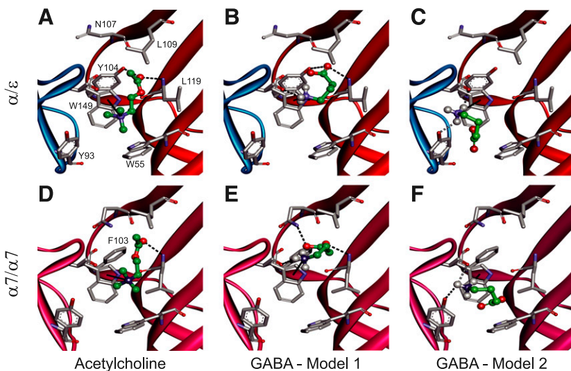
Fig. 5. Molecular docking of ACh or GABA to muscle \alpha/\epsilon (top) or \alpha 7/\alpha 7 (bottom) interfaces. Homology models of \alpha/\epsilon (A–C) (Supplemental Material; \alpha - \epsilon interface) and \alpha 7/\alpha 7 interfaces (D–F) (Supplemental Material; \alpha 7 - \alpha 7 interface) were generated using the structure of the AChBP (PDB ID 1UW6), as described in the text. The subunits are colored cyan ( \alpha ), red ( \epsilon ), and pink ( \alpha 7 ), and the corresponding residue atoms are colored as follows: gray for C, violet for N, red for O, and light gray for H. ACh and GABA carbons are colored green. The labeled residues are conserved among interfaces, except F103 in the \alpha 7 subunit of the complementary face, which corresponds to Y104 in the \epsilon subunit. The interactions of ligands with important residues of the binding site are also shown. Hydrogen bonds are shown with black dashed lines and cation- \pi interactions with solid lines.
