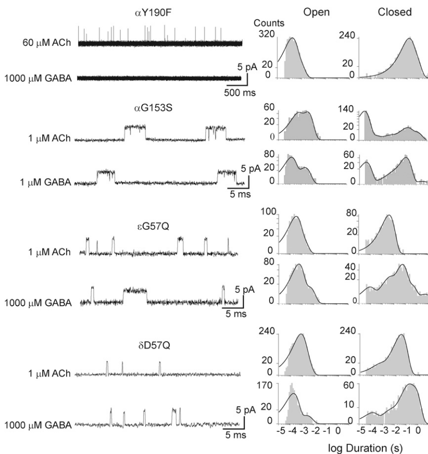
Fig. 2. Activation of mutant muscle nAChRs by GABA. Left, channels were recorded from BOSC 23 cells expressing nAChR containing the mutant \alpha Y190F, \alpha G153S, \epsilon G57Q, or \delta D57Q subunits. Currents are shown at a bandwidth of 7 kHz with channel openings as upward deflections. Right, open and closed time histograms of nAChRs carrying the specified mutant subunit. The data are representative of four to six recordings for each condition. Membrane potential: -70 mV.
