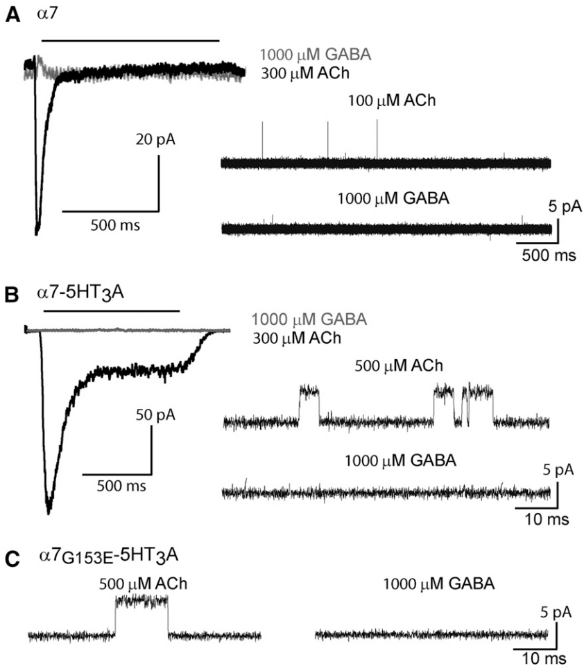
Fig. 4. Action of GABA on \alpha 7 nAChR. (A and B) Left, macroscopic current recordings activated by 1000 \mu\text{M} GABA (gray line) or 300 \mu\text{M} ACh (black line) from cells expressing \alpha 7 (A) or \alpha 7 -5HT 3 A receptors (B). The solid line above the traces represents the pulse of agonist. Each trace is representative of four recordings for each condition. Membrane potential: -70 mV. Right, single-channel traces from cells expressing \alpha 7 (A) or \alpha 7 -5HT 3 A receptors (B). Traces of currents are shown at a bandwidth of 7 kHz with channel openings as upward deflections. The data are representative of 10 or 20 recordings for each condition. Membrane potential: -70 mV. (C) Single-channel traces corresponding to \alpha 7 -5HT 3 A receptors carrying the \alpha 7 G153E mutation activated by 500 \mu\text{M} ACh or 1000 \mu\text{M} GABA (no channels detected, n = 13 ). Openings are shown as upward deflections at a bandwidth of 9 kHz. Membrane potential: -70 mV.
