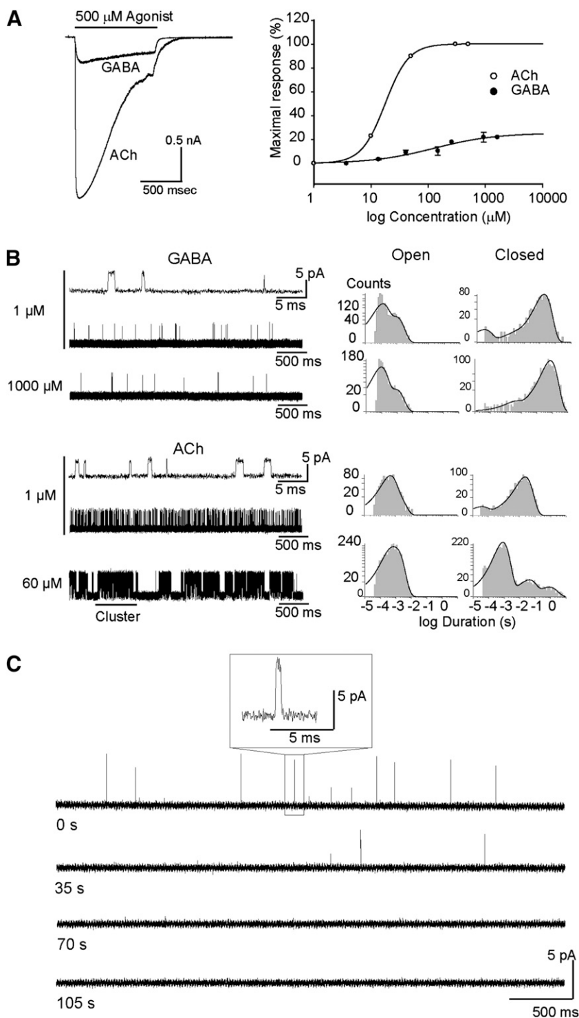
Fig. 1. Activation of adult muscle nAChR by GABA. (A) Left, whole-cell currents recorded in response to rapid perfusion of 500 \mu\text{M} ACh or 500 \mu\text{M} GABA. The solid bar indicates the duration of exposure to the drug. Each curve is the average of two to four drug applications. Right, dose-response curves for ACh (open symbols) and GABA (solid symbols) of muscle nAChR. Each point is the average of three to five determinations, with the error bars representing the S.D. of the mean value. Curves are fits to the Hill equation. Membrane potential: -70 mV. (B) Single channels activated by 1 and 1000 \mu\text{M} GABA and 1 and 60 \mu\text{M} ACh recorded from cells expressing adult muscle nAChR. Left, traces of currents are shown at a bandwidth of 10 kHz with channel openings as upward deflections. Right, open and closed time histograms corresponding to each condition. Membrane potential: -70 mV. (C) Single-channel recordings activated by 1000 \mu\text{M} GABA and 1 \mu\text{M} \alpha -BTX were recorded from cells expressing adult muscle nAChR. The tip of the pipette was filled with a solution containing only GABA, and the shaft with the solution containing GABA and \alpha -BTX. After the first minute of recording, a marked decrease of channel activity was observed. Traces are shown at a bandwidth of 7 kHz with channel openings as upward deflections. The inset shows an opening event at higher time resolution. Membrane potential: -70 mV.
