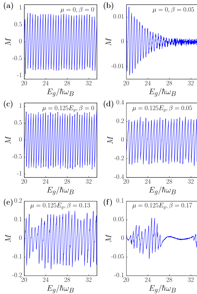
Figure 5. The QO of the magnetization at zero temperature for a set of values for the chemical potential and anisotropy parameter \beta . As discussed in the text, the ratio of the minimum direct bulk gap E_g and the LL spacing of the unhybridized itinerant electron band \hbar\omega_B for given magnetic field B provides a measure of the contributions to the magnetic oscillations from the gapped bulk. The latter become important for E_g/\hbar\omega_B \ll 1 . By contrast, we observe QO well above this threshold, due to the contribution of the surface states. Note that the chemical potential is always in the bulk gap. All other parameters are the same as in figure 1.
