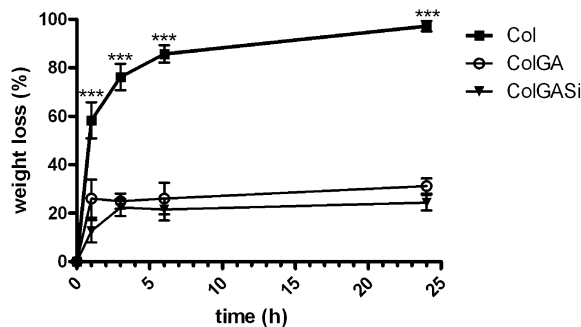
Fig. 6 Accelerated enzymatic degradation of acellular scaffolds by collagenase digestion. Weight percentage loss is shown as a function of time for pure collagen (Col), glutaraldehyde crosslinked (ColGA) collagen and silica-coated collagen hydrogels (ColGASi) data represented as mean (SD, n = 3 ).
