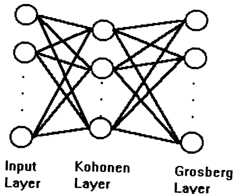
Figure 3. Counterpropagation Network
