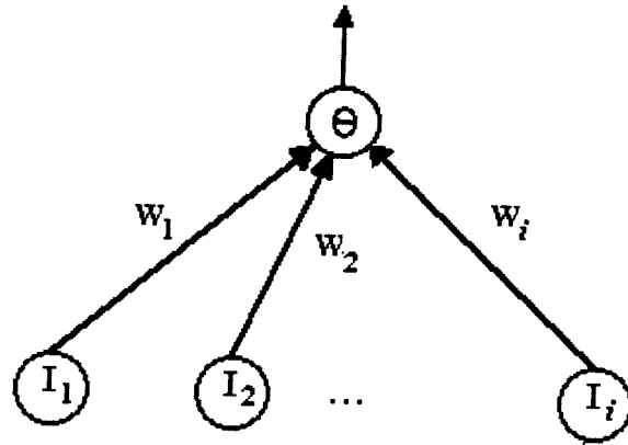
Figure 1. Simple Perceptron
