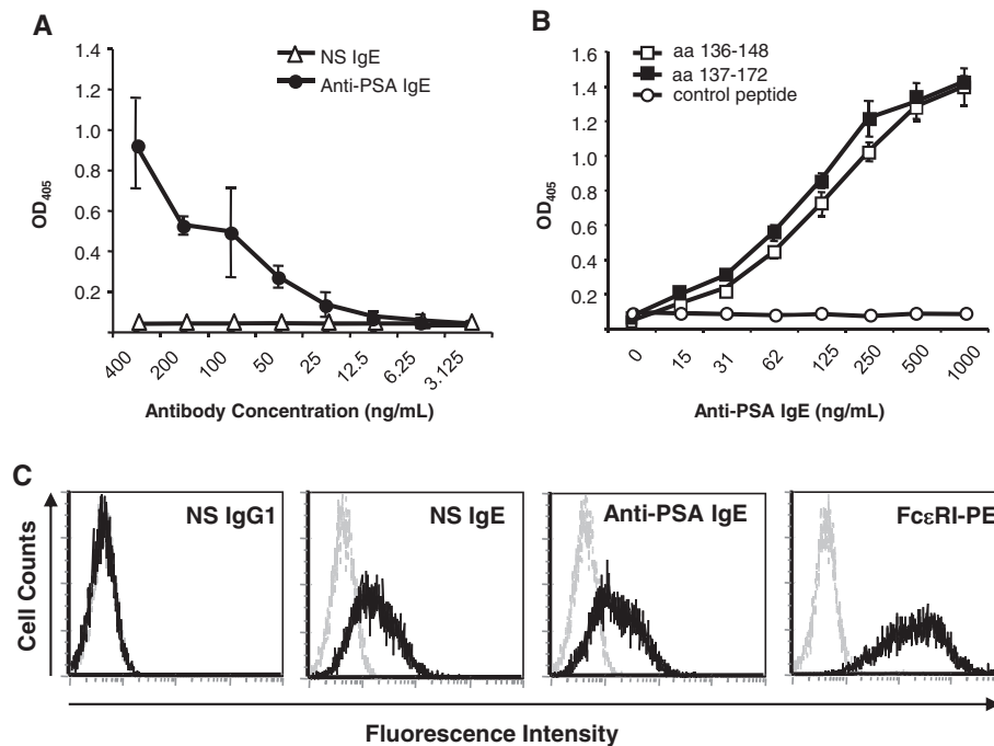
Figure 1 Binding to antigen and FcεRIα. A ) Binding of the anti-PSA IgE compared to a NS IgE to PSA was detected by ELISA. B ) Binding to the known epitope recognized by AR47.47 was confirmed by ELISA using PSA peptides containing the antigen binding site. Binding was detected by an AP-conjugated anti-human κ secondary antibody followed by a phosphatase substrate. ELISA data are the mean of triplicate samples with standard deviations indicated and are representative of 3 independent experiments. C ) Binding to the FcεRIα on the surface of CHO-3D10 cells was detected using flow cytometry and an anti-human κ FITC-conjugated antibody. An anti-FcεRI PE-conjugated antibody was used simultaneously to verify receptor expression. Data are representative of 3 independent experiments.
