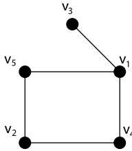
Fig. 2. The apple A_4 .
