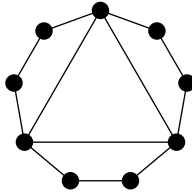
Fig. 1. The complement \bar{G} of a perfect graph G such that T(G) is not perfect, independently of the orientation of \bar{G} .
