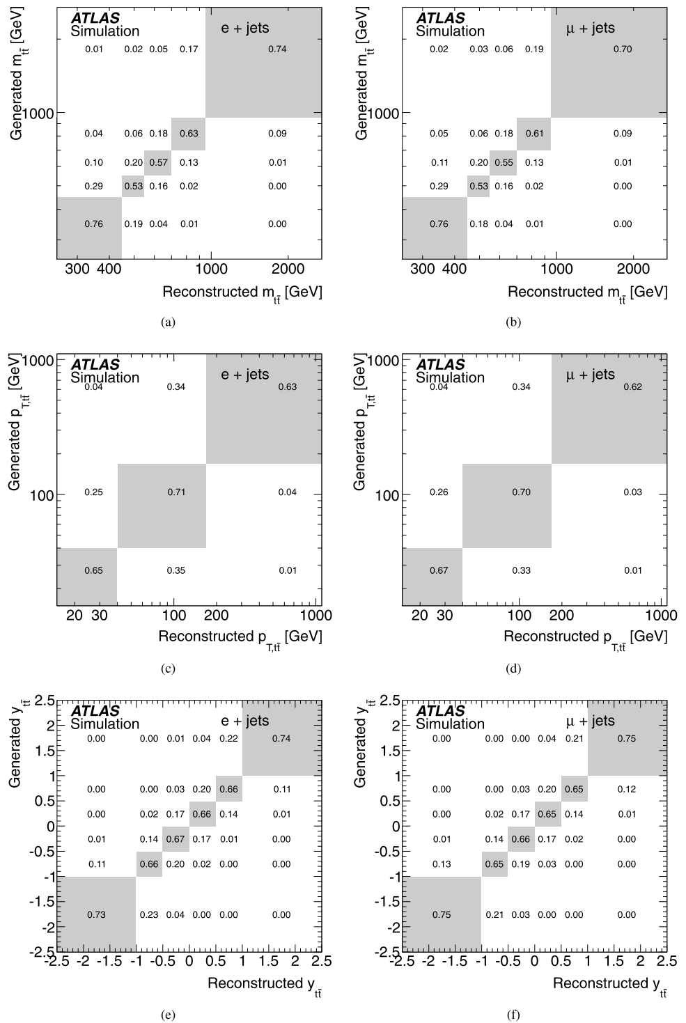
Fig. 3 Migration matrices for (a–b) m_{T,\bar{t}t} , (c–d) p_{T,\bar{t}t} , and (e–f) y_{\bar{t}t} estimated from simulated t\bar{t} events passing all (left) e + \text{jets} and (right) \mu + \text{jets} selection criteria. The unit of the matrix elements is the probability for an event generated at a given value to be reconstructed at another value
