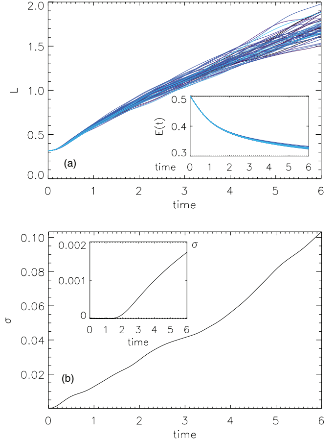
FIG. 3. (Color online) (a) Time evolution of the integral scale for all the 2048^2 runs; note the dispersion around the mean evolution. The inset shows the time evolution of the energy for all runs, which are very close. (b) Time evolution of the standard deviation \sigma in the integral scale of all the 2048^2 runs. The inset shows the standard deviation in the energy in all the 2048^2 runs as a function of time.
