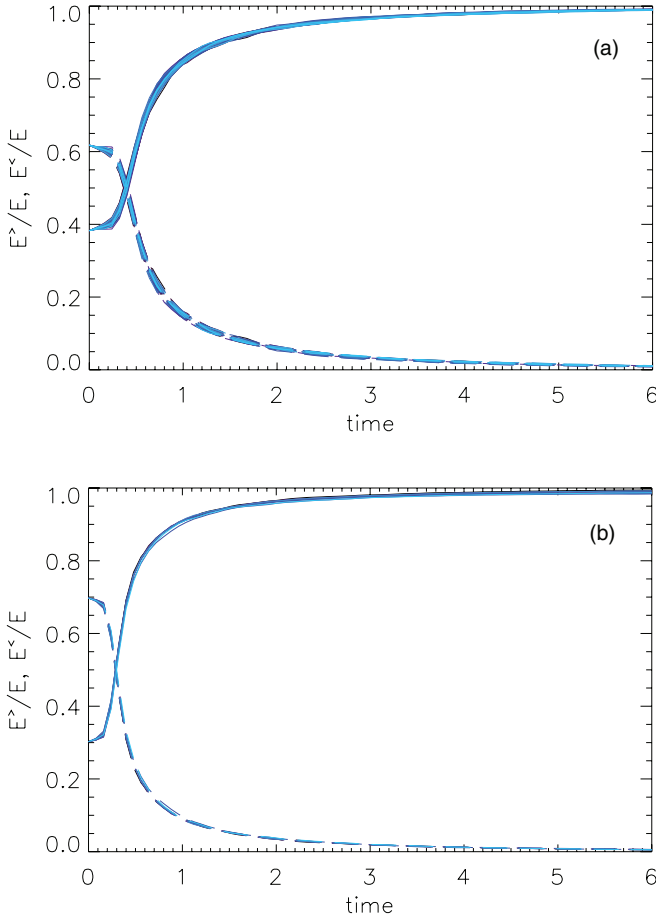
FIG. 2. (Color online) Time evolution of E^</E (solid line) and E^>/E (dashed line) (ratio of the energy at large and small scales, respectively, to the total energy) as a function of time for all runs in the set of simulations with (a) 2048^2 grid points and (b) 4096^2 grid points.
