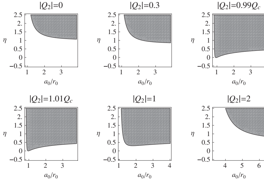
FIG. 5. Shell around a black hole in Einstein-Born-Infeld theory with b/r_0 = 1 . The values of the parameters are \Lambda r_0^2 = -1 , M_1 = 0.16 , Q_1 = 0 , M_2 = 0.8 ; the critical value of the charge is Q_c = 0.8944 .
