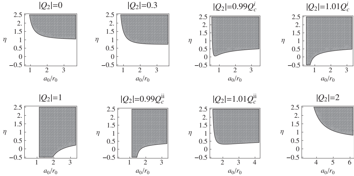
FIG. 4. Shell around a black hole in Einstein-Born-Infeld theory with b/r_0 = 1 . The values of the parameters are \Lambda r_0^2 = -1 , M_1 = 0.1 , Q_1 = 0 , M_2 = 0.5 ; the critical values of the charge are Q_c^i = 0.4657 and Q_c^{ii} = 1.2597 .
