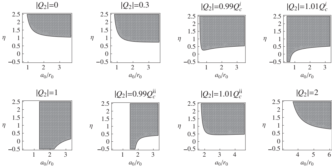
FIG. 1. Shell around a black hole in Einstein-Maxwell theory. The values of the parameters are \Lambda r_0^2 = -1 , M_1 = 0.1 , Q_1 = 0 , M_2 = 0.5 ; the critical values of the charge are Q_c^i = 0.4321 and Q_c^{ii} = 1.4682 .
