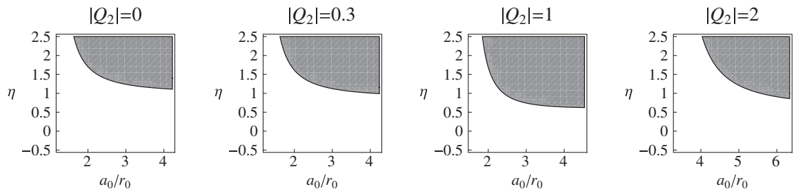
FIG. 3. Shell around a black hole in Einstein-Maxwell theory. The values of the parameters are \Lambda r_0^2 = -1 , M_1 = 0.3 , Q_1 = 0 , M_2 = 1.5 .
