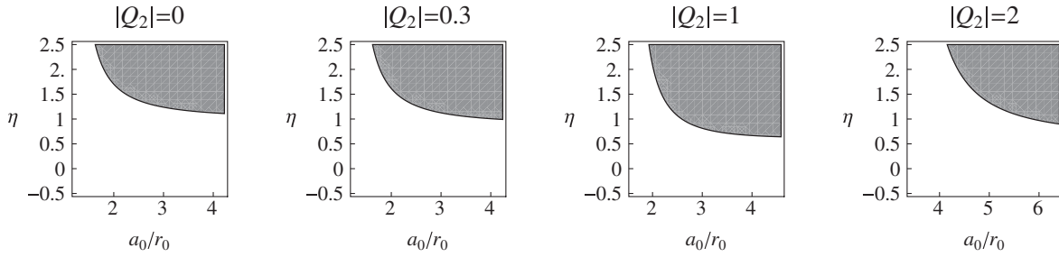
FIG. 6. Shell around a black hole in Einstein-Born-Infeld theory with b/r_0 = 1 . The values of the parameters are \Lambda r_0^2 = -1 , M_1 = 0.3 , Q_1 = 0 , M_2 = 1.5 .
