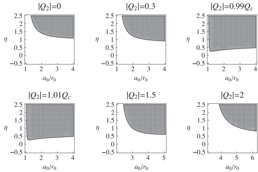
FIG. 2. Shell around a black hole in Einstein-Maxwell theory. The values of the parameters are \Lambda r_0^2 = -1 , M_1 = 0.2 , Q_1 = 0 , M_2 = 1 ; the critical value of the charge is Q_c = 1 .
