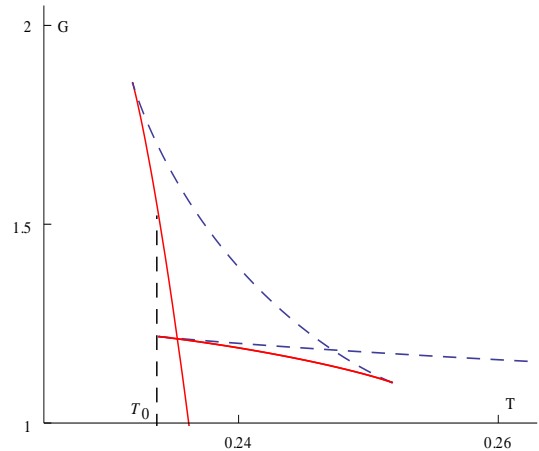
FIG. 3. Zeroth order phase transition in d = 6 . A close-up of fig. 2 illustrating the discontinuity in the global minimum of G at T = T_0 \approx 0.2339 \in (T_t, T_z) (denoted by the vertical line). We have set P = 0.0564 \in (P_t, P_z) and J = 1 . Solid-red/dashed-blue lines correspond to C_P positive/negative respectively.
