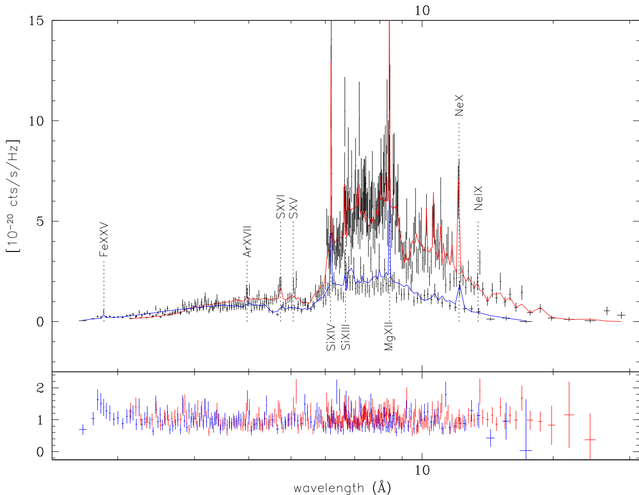
Figure 1. Top panel: MEG data and their best fit model (red line) & HEG data and their best fit model (blue line). Bottom panel: data/model ratio, with the same color convention as above. Note that the wavelength scale is logarithmic.
