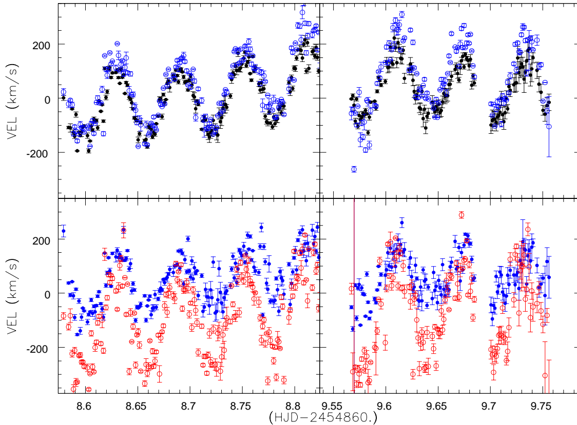
Figure 3. Top panels: radial velocity curves of the emission lines H \beta (black solid circles) and H \gamma (blue circles) during the Feb 6 (left) and Feb 7 (right) observing runs. Bottom panels: radial velocity curve of the emission lines He II \lambda 4686 (blue solid circles) and the C III + N III blend (red circles) during the same nights. The y range is the same in all the panels.
