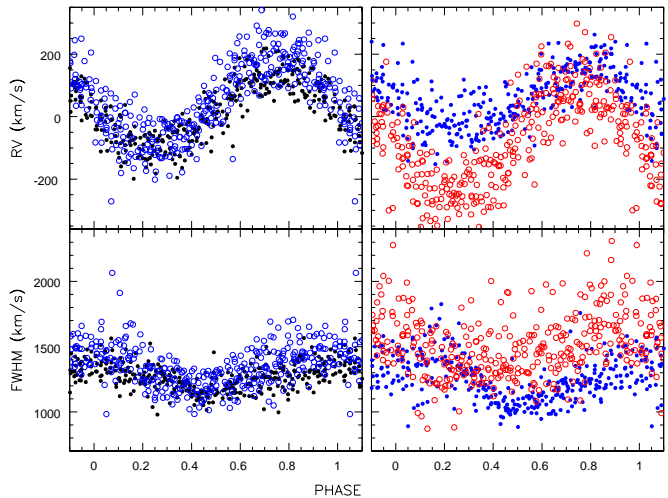
Figure 4. Top panels: radial velocity curve of the emission lines H\beta and H\gamma (left) and \text{He II} and \text{C III} (right - same color code as in Fig. 3). Bottom panels: modulation of the emission lines FWHM with the \sim 1.47 hr period. Note that while H\beta and H\gamma FWHM present an almost sinusoidal modulation, the \text{He II} modulation is more similar to a sawtooth profile. The \text{C III} FWHM is much less modulated and “noisy”, possibly indicating a variable contribution/blend with the \text{N III} emission line.
