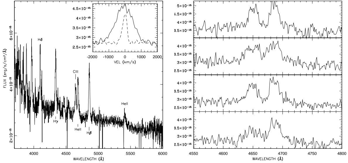
Figure 2. Left panels: a representative spectrum of our time series. It has been obtained by averaging two spectra taken toward the end of the first night. Note that the spikes at 4130 4517 5018 5065 5395 and 5665 Å are all bad pixels. The inset compare the H \beta line profile (solid line) with that of the sky emission lines O I \lambda 5577 (dashed line). Right panel: example of profile variation shown by the C III and He II emission lines. The four spectra are separated by about 25-50 minutes each other.
