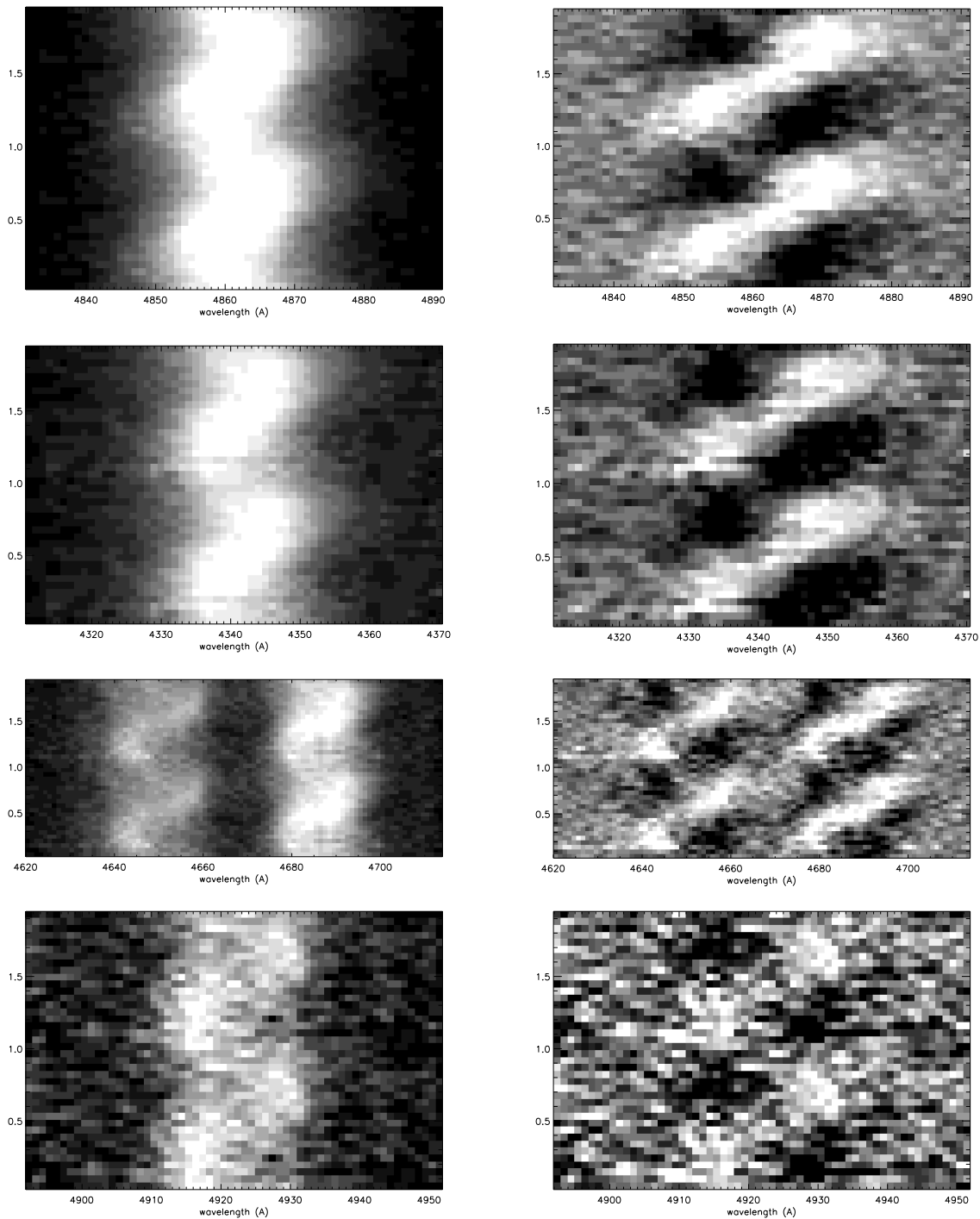
Figure 5. Trailed spectra (left panels) and “difference trailed spectra” (right panels) of the emission lines H\beta , H\gamma , He\ II + C\ III and He\ I , from top to bottom. Phase 0 corresponds to the time for the red-to-blue crossing in the high-frequency modulation.
