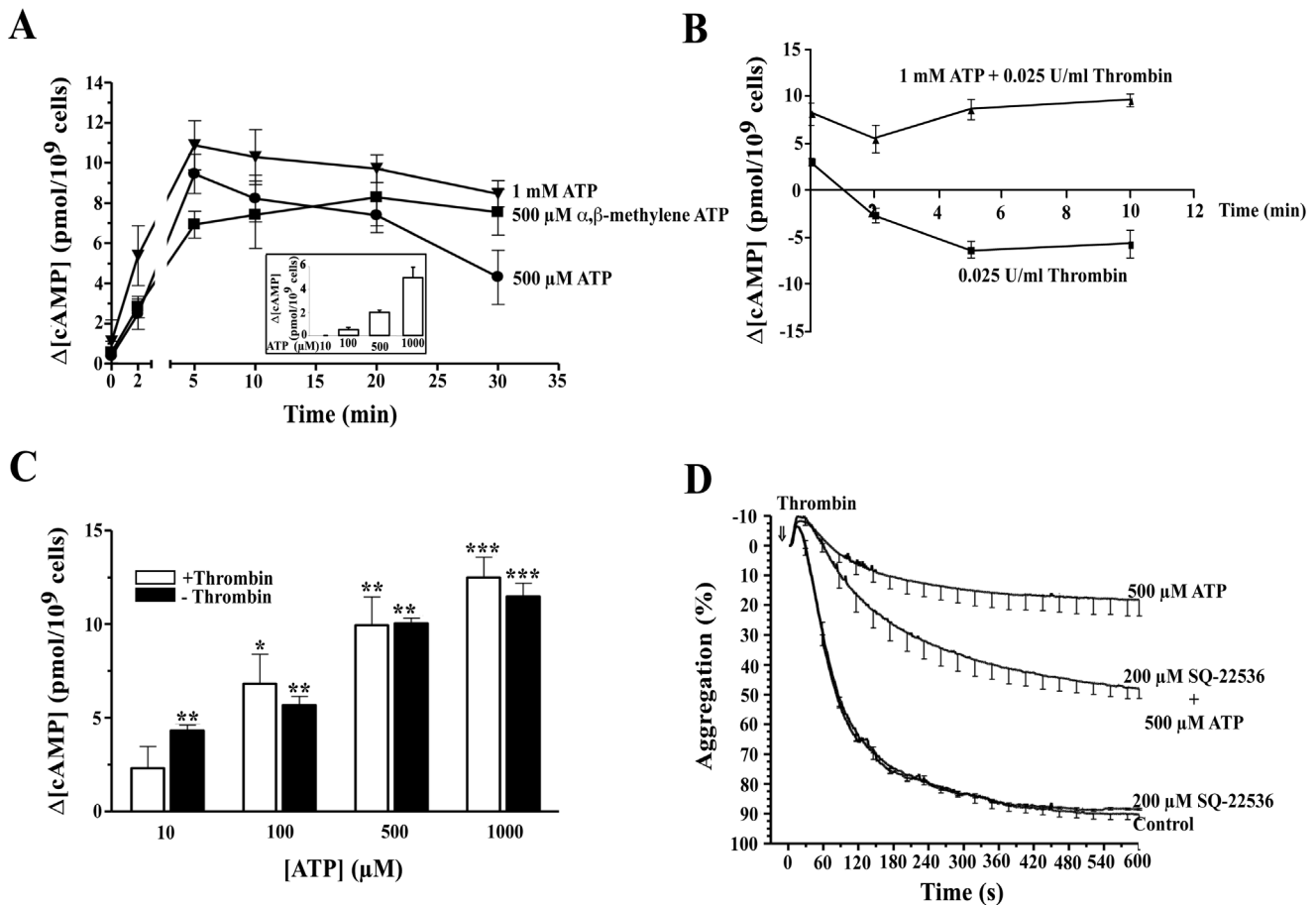
Figure 7. Effect of ATP on the cAMP levels in human platelets. (A) Washed human platelets were preincubated with a mixture of phosphodiesterase inhibitors for 5 min at 37°C, as indicated in Materials and Methods. Then, cells were incubated with 500 μM (●) or 1 mM (▼) ATP, (■) 500 μM α,β-methylene ATP or vehicle for 2, 5, 10, 20 and 30 min. Inset, Washed human platelets were incubated with different concentrations of ATP for 5 min at 37°C in the absence of phosphodiesterase inhibitors. The reactions were stopped by addition of ice-cold TCA (10% final concentration). The cAMP levels were determined as described in Materials and Methods. Data represent the means ± s.e.m of 5 (A) and 3 (inset) experiments with different platelets preparations, performed in duplicate and assayed in triplicate. (B) Washed human platelets were preincubated with a mixture of phosphodiesterase inhibitors for 5 min at 37°C, as indicated in Materials and Methods. Then, cells were incubated with or without 1 mM ATP for 5 min at 37°C. Finally, cells were stimulated with 0.025 U/ml for 0, 2, 5 and 10 min in the presence of 1 mM CaCl 2 . The reaction was stopped by addition of ice-cold TCA (10% final concentration). The cAMP levels were determined as described in Materials and Methods. Data are the means ± s.e.m of 5 experiments with different platelets preparations, performed in duplicate and assayed in triplicate. (C) Washed human platelets were also preincubated with a mixture of phosphodiesterase inhibitors for 5 min followed by incubation in the presence of various concentrations of ATP or vehicle for 5 min and finally stimulated with 0.025 U/ml thrombin or vehicle for 5 min in the presence of 1 mM CaCl 2 . The reaction was stopped by addition of ice-cold TCA (10% final concentration). The cAMP levels were determined as described in Materials and Methods. Data are the means ± s.e.m of 5 experiments with different platelets preparations, performed in duplicate and assayed in triplicate. *P<0.05, **P<0.01, ***P<0.001. (D) Washed human platelets were preincubated with 200 μM SQ-22536 or vehicle for 2 min. Then, cells were incubated with 500 μM ATP or vehicle for additionally 2 min. Finally, cells were stimulated with 0.025 U/ml thrombin (↓, time=0). The aggregation was measured for 10 min and values represent the average curves of aggregation (% mean±s.e.m) of 4 experiments with different platelet preparations. doi:10.1371/journal.pone.0067117.g007
