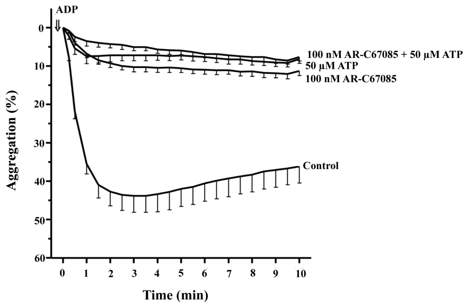
Figure 3. Effect of A_3P_5P and AR-C67085 on ADP-induced platelet aggregation. Washed human platelets were preincubated with (A) 200 \mu M A_3P_5P or vehicle for 10 min and (B) with 100 nM AR-C67085 or vehicle for 10 min. Then, cells were incubated with 50 \mu M ATP or vehicle for 2 min. Finally, cells were stimulated with 10 \mu M ADP ( \downarrow , time=0) in the presence of 0.3 mg/ml fibrinogen (added 1 minute before ADP). The assay was performed in the presence of 1 mM CaCl_2 . The aggregation was measured for 10 min and values represent the average curves of aggregation (% means \pm s.e.m) of 5 experiments with different platelet preparations. doi:10.1371/journal.pone.0067117.g003
