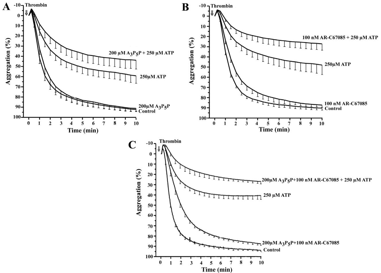
Figure 4. Effect of ADP receptor antagonists on the TIPA inhibition mediated by ATP. Washed human platelets were preincubated with (A) 200 \mu\text{M} \text{A}_3\text{P}_5\text{P} or vehicle for 10 min, (B) 100 nM AR-C67085 or vehicle for 10 min and (C) 200 \mu\text{M} \text{A}_3\text{P}_5\text{P} + 100 nM AR-C67085 or vehicle for 10 min. Then, cells were incubated in the presence of ATP or vehicle for 2 min. Finally, cells were stimulated with 0.025 U/ml thrombin ( \Downarrow , time = 0). The aggregation was measured for 10 minutes and values represent the average curves of aggregation (%), means \pm s.e.m) of 5 experiments with different platelet preparations. doi:10.1371/journal.pone.0067117.g004
