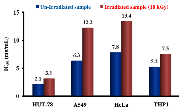
Fig. 4. IC_{50} value of F3 from ethyl acetate extract of unirradiated and irradiated samples at 10 kGy against human cancer cell lines (HUT78, A549, HeLa, THP1).
