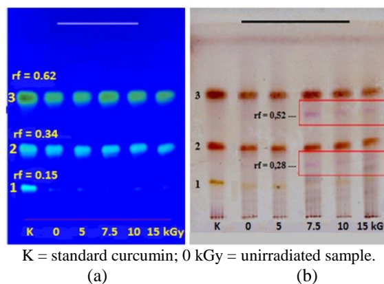
Fig. 2. Thin-layer chromatogram (TLC) of F3 from varying irradiation dose compared to the standard curcumin; (a) spots on the TLC plate under the UV lamp with λ 366 nm; (b) the TLC plate after spraying with reagent cerium sulfate and heating.
