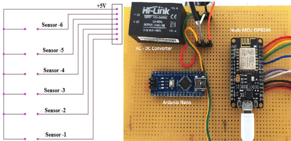
Fig. 4 — Sensor array connection diagram with fabricated mother board
