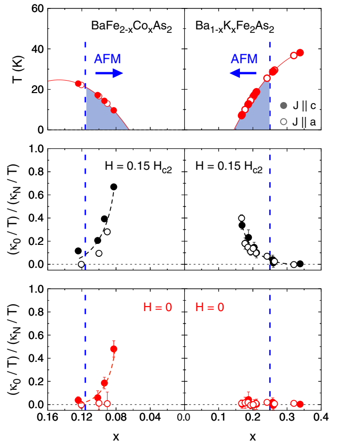
FIG. 7. Comparison of the superconducting gap anisotropy determined from thermal conductivity studies in electron-doped Co-Ba122 (left column) [19,20] and hole-doped K-Ba122 (right column, this work). The top panels show the phase diagrams of both materials. The middle and bottom panels show \kappa_0/\kappa_N vs x for H = 0.15 H_{c2} and H = 0 , respectively. Open (closed) symbols correspond to transport along J||a ( J||c ).
