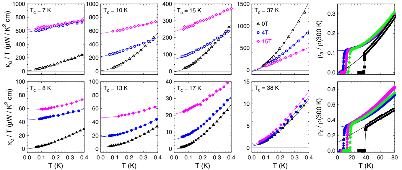
FIG. 1. Thermal conductivity of K-Ba122 at four representative K concentrations, indicated by their T_c values, plotted as \kappa/T vs T for in-plane ( \kappa_a , top panels) and interplane ( \kappa_c , bottom panels) directions of the heat current. Data are shown for three values of the magnetic field, as indicated (data for other fields are not shown for clarity). Lines are fits to \kappa/T = a + bT^\alpha , used to extract the residual linear term a \equiv \kappa_0/T . The rightmost panels show the electrical resistivity of the same samples, normalized to its value at T = 300 K, as a function of temperature. The line is a fit to the data at low temperatures, extended to T = 0 to extract the residual resistivity \rho_0 . For clarity, only the fits for samples with T_c \cong 7 and 38 K are shown.
