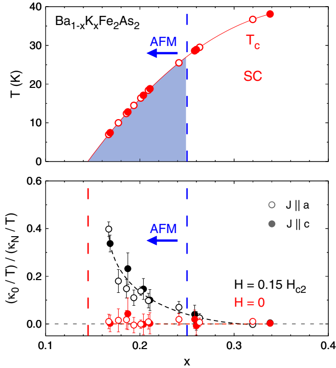
FIG. 4. Top panel: Doping phase diagram of K-Ba122, showing the onset of the superconducting phase (SC) below the critical temperature T_c as a function of the K concentration (doping) x . Open (closed) red circles give the T_c values of the a -axis ( c -axis) samples used in this study. For compositions to the left of the dashed blue line at x \simeq 0.25 ( T_c \simeq 26 K) [38,53], superconductivity coexists with antiferromagnetism (AFM). Bottom: Residual linear term in the thermal conductivity \kappa as T \rightarrow 0 , \kappa_0/T , plotted as a fraction of the normal-state conductivity, \kappa_N/T , for both \kappa_a (open symbols) and \kappa_c (closed symbols), for magnetic fields H = 0 (red) and H = 0.15H_{c2} (black). Error bars reflect the combined uncertainties of extrapolating \kappa/T and \rho to T = 0 , to get \kappa_0/T and \rho_0 . The red vertical dashed line at x = 0.15 marks the end of the superconducting phase.
