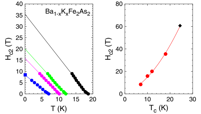
FIG. 3. Left panel: Upper critical field H_{c2}(T) for H \parallel c , as a function of temperature, for four samples, with T_c = 7 K (blue), 10 (magenta), 12 (green), and 19 K (black). H_{c2} is determined from electrical resistivity measurements [41]. The blue square shows the H_{c2} value determined from thermal conductivity measurements on the T_c = 7 K sample. The lines are a linear fit of each data set, extrapolated to T = 0 . The value of H_{c2} thus extrapolated to T = 0 , H_{c2}(0) \equiv H_{c2} , is plotted vs x in the right panel. Right panel: H_{c2}(0) vs T_c from data in the left panel (red dots), plus one point at high doping from published data (black diamond) [41]. The line is a polynomial fit of the data, used to extract the values of H_{c2} for the samples T_c between 7 and 25 K.
