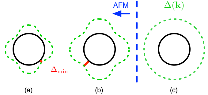
FIG. 5. Sketch of the evolution of the gap structure in K-Ba122 with doping x , where the gap (green dash line) is shown around a single Fermi surface (black circle). The gap is isotropic at optimal doping (c). The modulation of the gap starts upon entering the region where antiferromagnetism (AFM) appears, and coexists with superconductivity (panel b). The gap minimum deepens with decreasing x (panel a).
