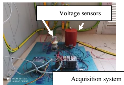
Figure 2. Measurement setup arranged in the DC substation. Scheme a) and picture a) of the setup.
