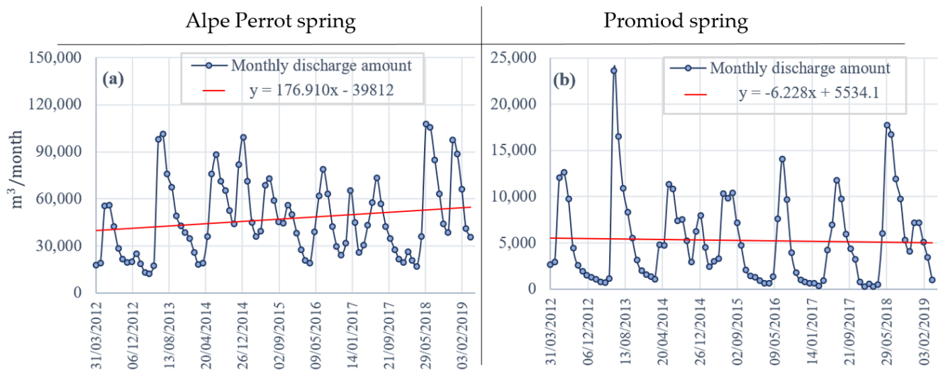
Figure 8. Time series of discharge (a,b) of the two sets of best-correlated weather station—springs study cases: Alpe Perrot—Champdepraz (a) and Promiod—Saint Vincent (b). The linear interpolation trend is represented by a red line and the regression equation is shown on each plot.
