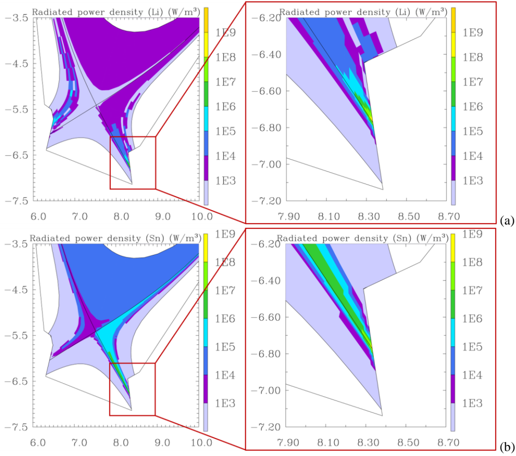
Figure 8. Computed 2D distributions of the radiated power density for Li (a) and Sn (b), for the case n_{e,sep} = 4.5 \cdot 10^{19} \text{ m}^{-3} , with an enlargement showing the conditions in front of the OT.
