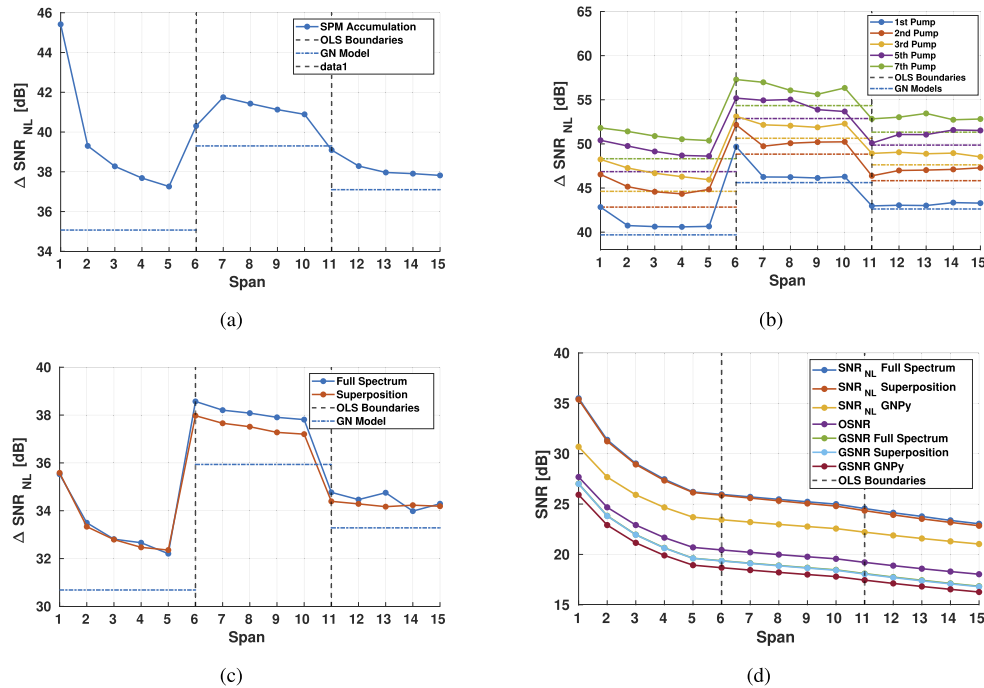
Fig. 5. The gradient of the SNR_{NL} accumulation, \Delta SNR_{NL} , for Scenario 2. We present: (a) a single propagating channel, (b) 5 selected pump-and-probes, (c) a full spectrum transmission scenario compared with that of a pump-and-probe superposition. In (d), the SNR_{NL} accumulation of (c) is shown, along with an OSNR calculated by considering ideal amplification, and the corresponding GSNRs for the full spectrum, superposition and GNPpy simulations.
