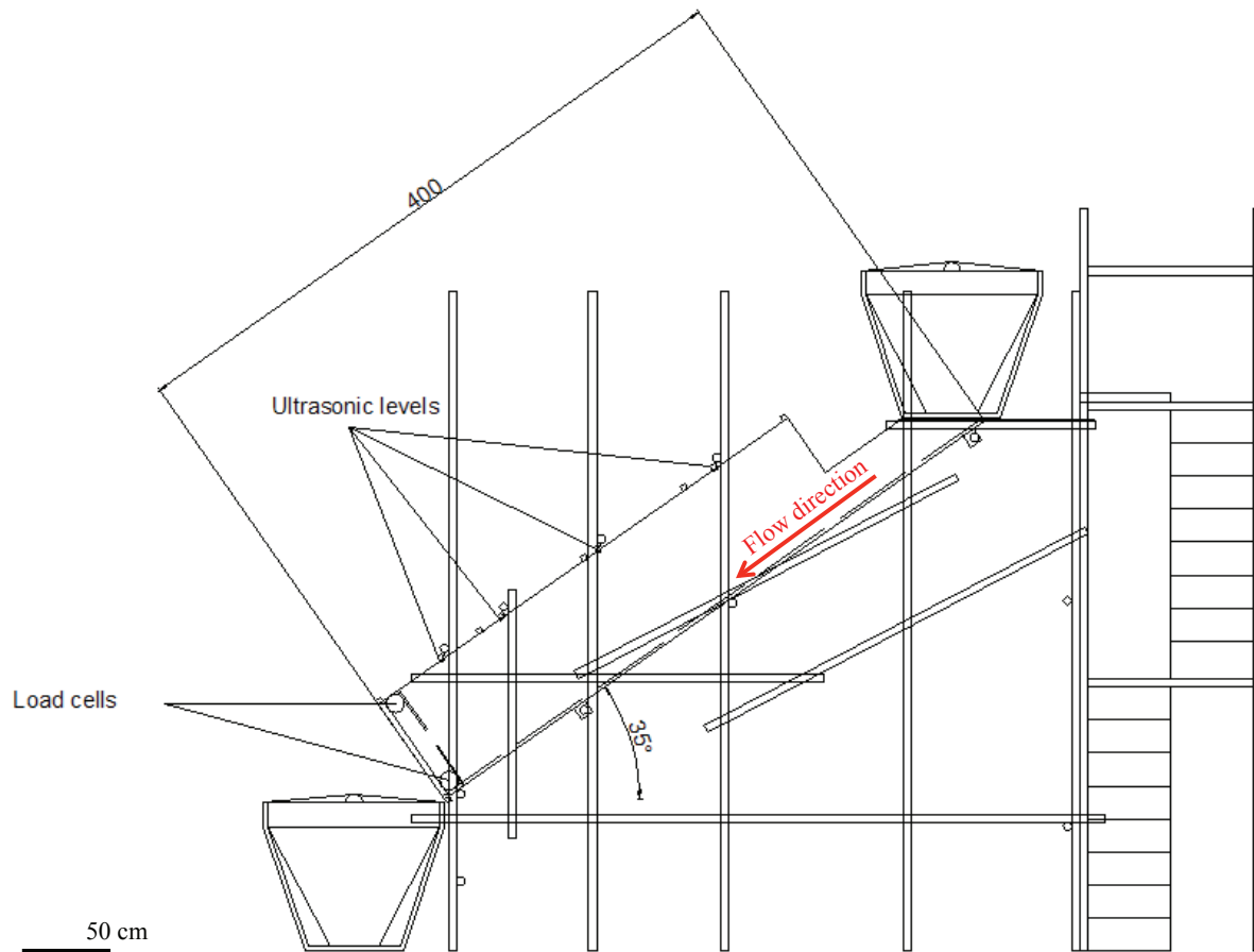
Figure 2. Schematic of the flume and of the starting mechanism.
