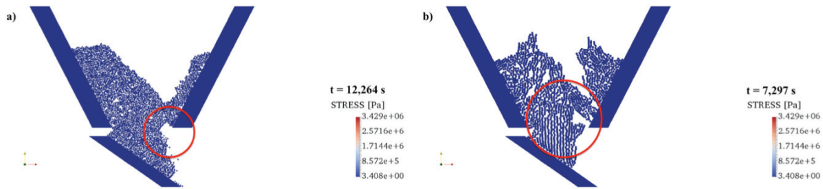
Figure 4. Particular of the releasing phase in numerical simulations using triangular particles (a) and square particles (b). Red circles highlight the formation of arch effects and vertical piling due to the particle shape.
