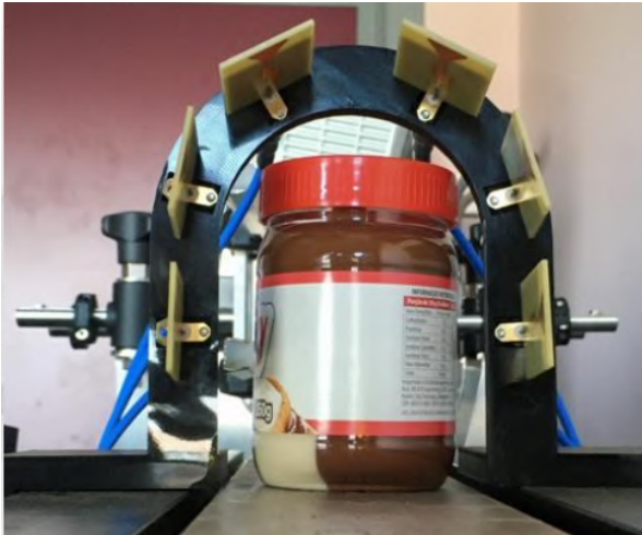
Fig. 1. Antennas array surrounding the item to inspect
