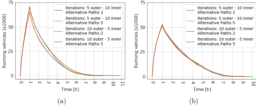
Figure 2.5: Stability study of SUE algorithm with (a) Gawron and (b) Logit methods.
