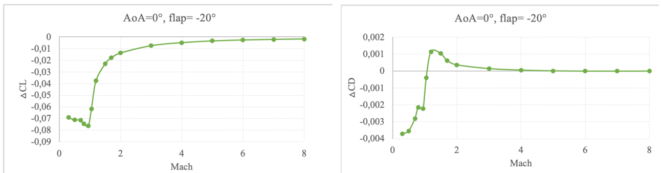
(a) (b) Figure 19 - \Delta C_L (a) and \Delta C_D (b) due to the flap effect at AoA=0^\circ and flap=-20^\circ .
