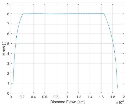
Figure 8 – Mach number vs Distance flown for clean external configuration
