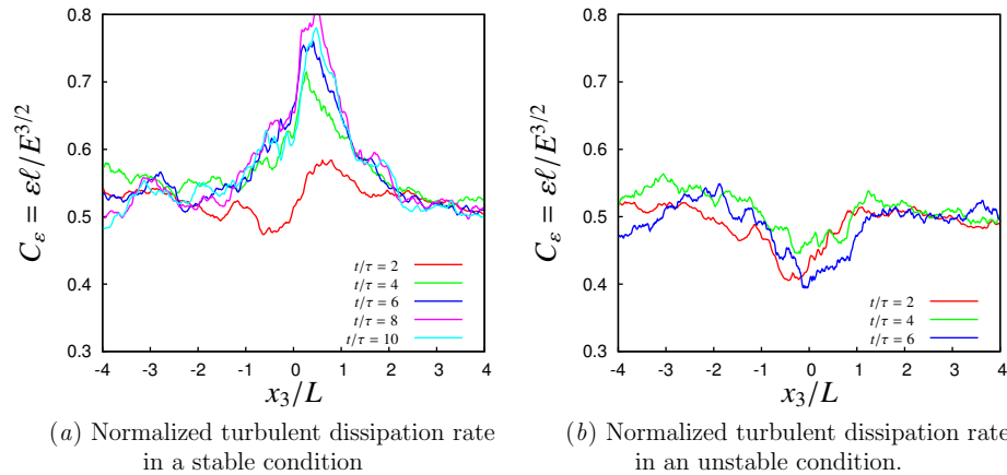
FIG. 21. (a,b) Normalized plane-averaged dissipation C_\varepsilon = \{\varepsilon\} \ell / \{E\}^{3/2} for Fr^2 = 4.0 and Fr^2 = -4.0 , respectively. Values outside the mixing layer are close to 0.5, as in the case of isotropic homogeneous turbulence 42 . In stable cases, the normalized dissipation shows a maximum at the kinetic energy pit; in an unstable case, the dissipation shows a minimum at the energy peak.
