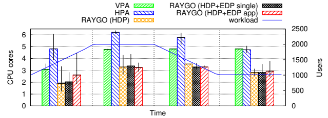
Figure 3. The sum of CPU requests assigned by each solution to the set of microservices, grouped by test phase.
