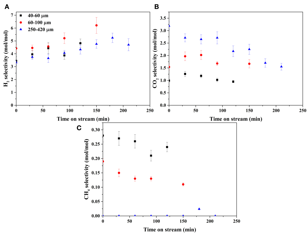
FIGURE 7 | Selectivities of gaseous products: (A) \text{H}_2 , (B) \text{CO}_2 , and (C) \text{CH}_4 .
