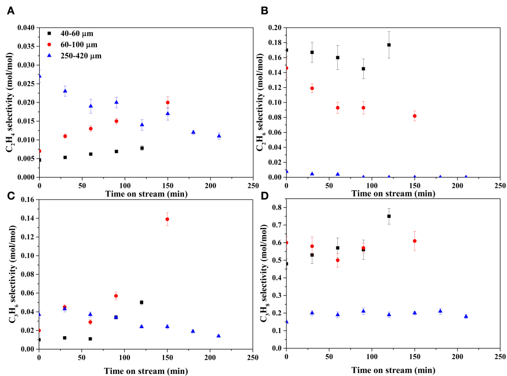
FIGURE 8 | Selectivities of \text{C}_{2-3} products. (A) ethylene, (B) ethane, (C) propylene, and (D) propane.
