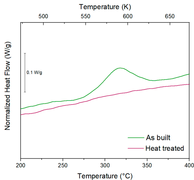
Figure 7. DSC signals of the as-built and heat-treated samples.
