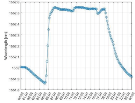
Fig. 4. Time evolution of the wavelength acquired in a whole day by the FBG sensor of the "Radiator" test equipment (10/01/2020).
