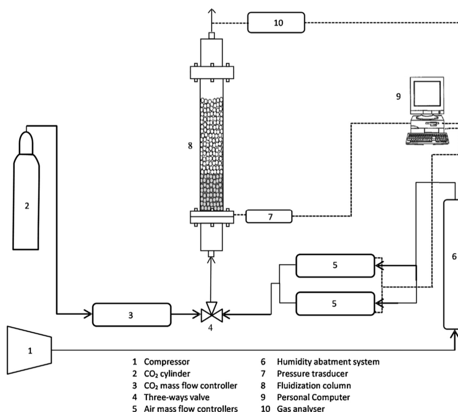
Figure 1. Experimental apparatus.
