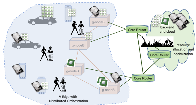
Figure 1. The V-Edge concept: Abstraction of the physical resources of the cloud back end, the 5G/6G core and RAN, as well as users and machines. All components provide (and may use) resources for edge computing and they may participate in a local, distributed orchestration on short time scales, while global optimization and other non-real-time operations can be performed in the cloud back end.
