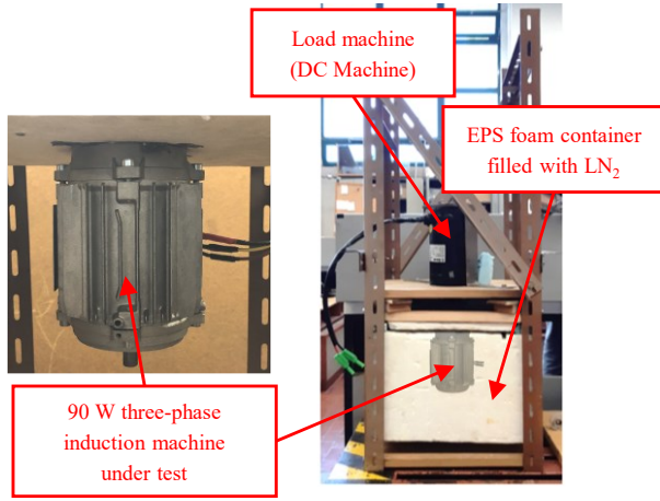
Fig. 8. The experimental setup developed to perform the room temperature and the cryogenic temperature tests on the 90 W machine. During the cryogenic test, the motor was placed into the EPS container and completely submerged by LN 2 .
