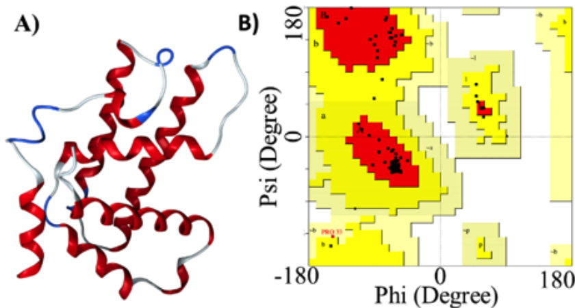
Figure 1. A) I-Tasser Homology model for the VPS9 (structured domain showed in New Cartoon representation); B) Rhamacdran Plot.
