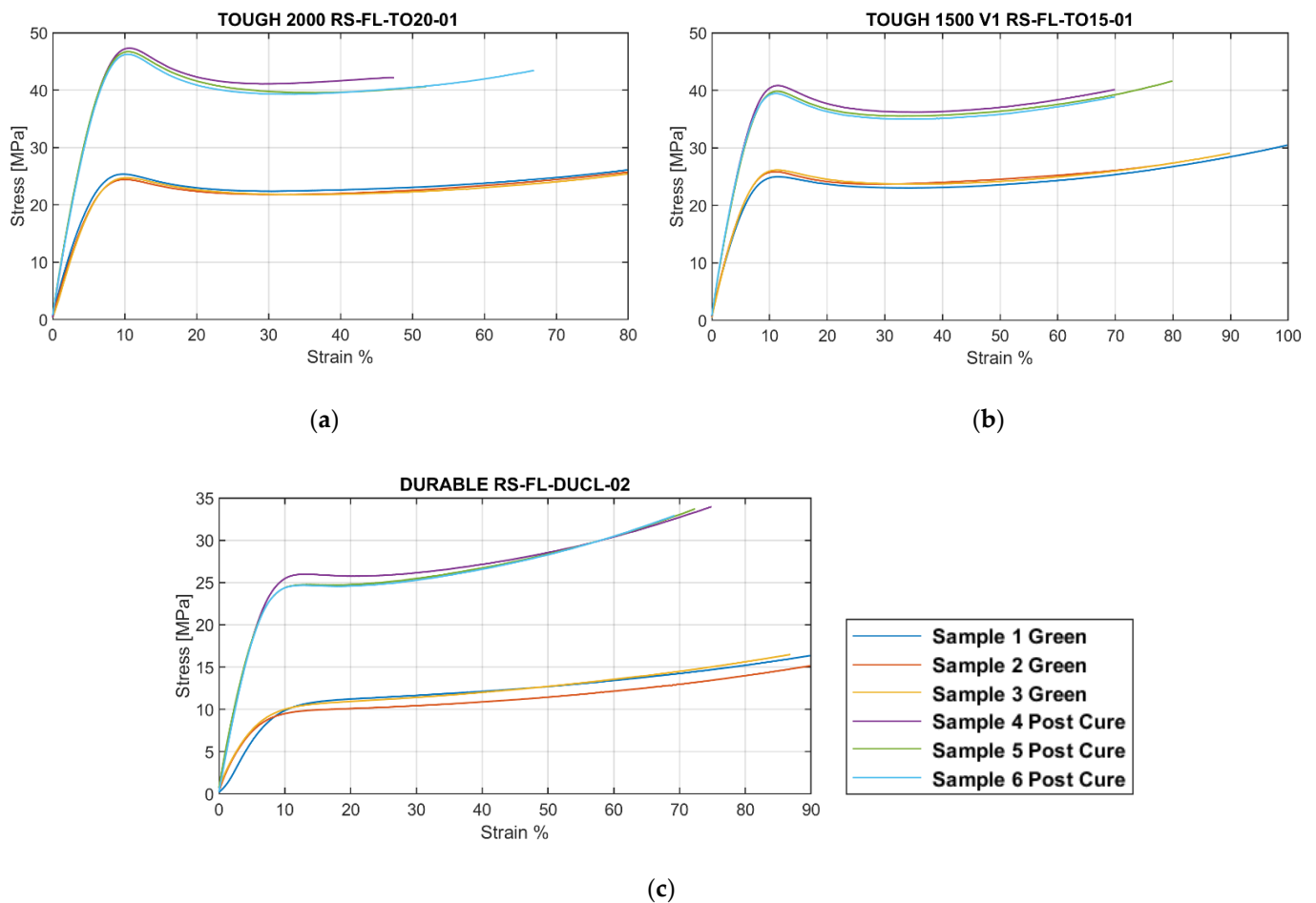
Figure 2. Stress-strain curve green and post-cure of Tough 2000 (a), Tough 1500 (b), and Durable (c) Resins. The legend of the stress-strain graphs, reported in the bottom row, is valid for each resin in the following figures also.
