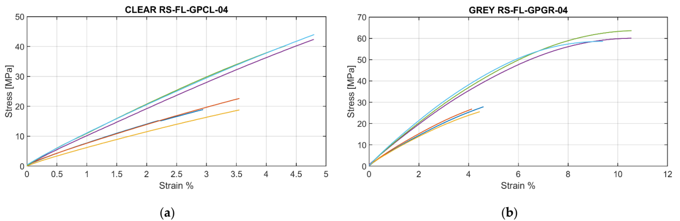
Figure 4. Stress-strain curve green and post-cure of Standard Clear (a) and Grey Pro (b) Resins. Lines are coloured as in Figure 2.
