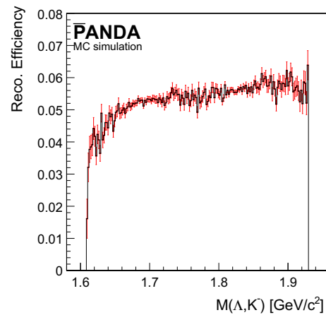
Fig. 11 Reconstruction efficiency (black histogram) as function of the invariant \Lambda K^- mass in the process \bar{p}p \rightarrow \bar{E}^+ \Lambda K^- . The statistical error is shown in red
