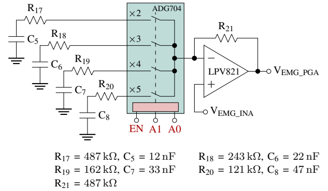
Fig. 10. Programmable Gain Amplifier (PGA): adaptable amplifier gains (i.e., \times 2 , \times 3 , \times 4 and \times 5 ) are obtained by controlling the analog multiplexer on the amplifier inverting branch.
