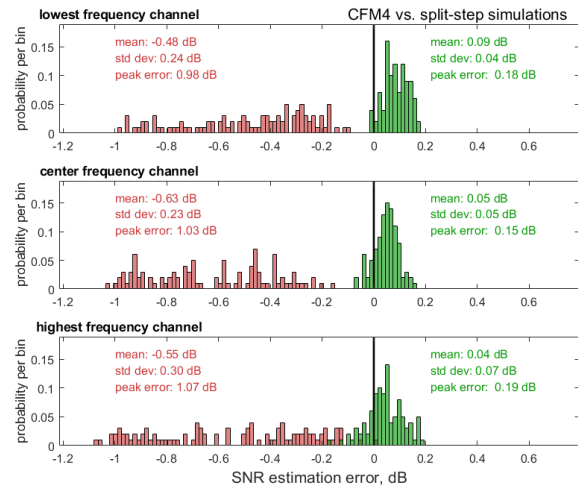
Fig. 11. Green bars: histograms of the SNR estimation error \Delta_{\text{SNR}}^{\text{dB}} between the closed-form model 4 (CFM4) and full C-band split-step simulations. The error is as defined by Eq. (8) and measured at maximum reach. The simulations were performed using systems randomly chosen among the 3150 PM-QAM systems of category (1). Each histogram was drawn based on 100 different systems. Red bars: CFM1 vs. simulations.
