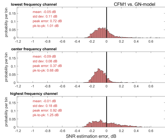
Fig. 4. Histograms of the SNR estimation error \Delta_{\text{SNR}}^{\text{dB}} between the closed-form model 1 (CFM1) and the GN-model, as defined by Eq. (8). The error is measured at maximum reach. Each histogram was built by looking at about 2800 different systems.
