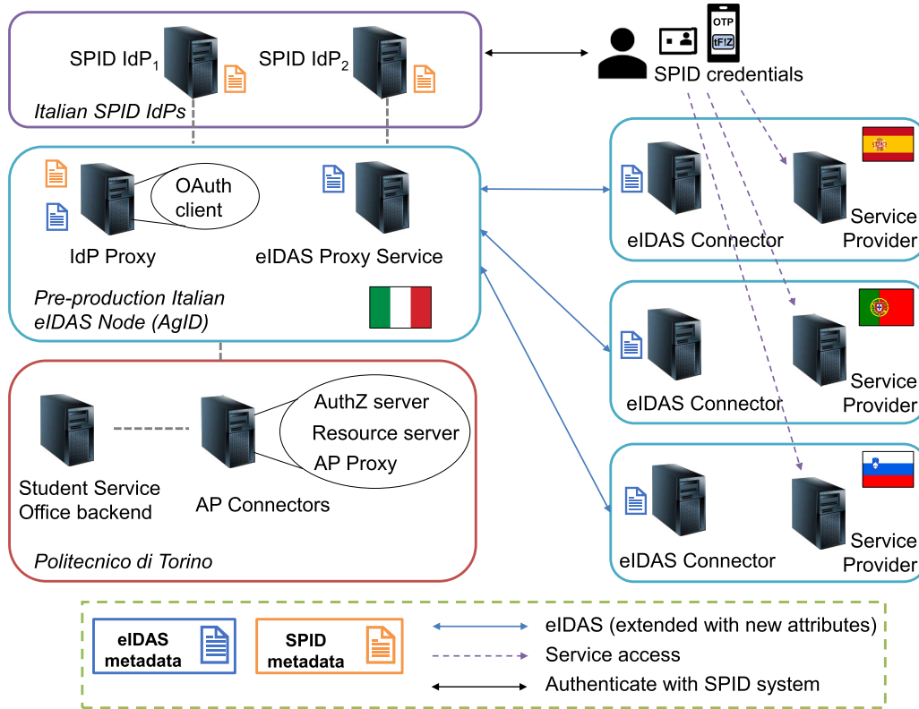
FIGURE 17. Experimental testbed.
