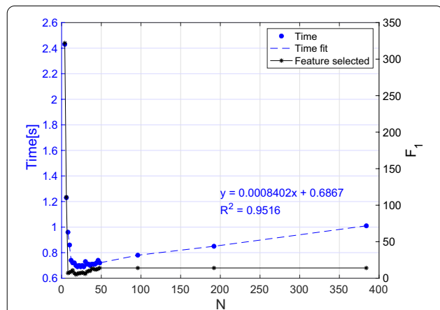
Fig. 5 Execution time of the algorithm with different numbers of inputs. The final number of features selected is also reported
