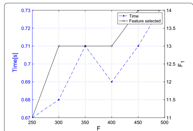
Fig. 7 Execution time of the algorithm with different numbers of input features. The final number of features selected is also reported
