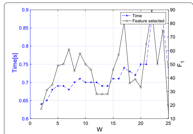
Fig. 6 Execution time of the algorithm with different numbers of words. The final number of features selected is also reported
