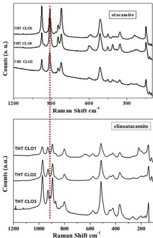
Figure 6. Raman spectra of copper trihydroxychlorides [Cu 2 Cl(OH) 3 ] atacamite and clinoatacamite on the coins found at Tharros.
