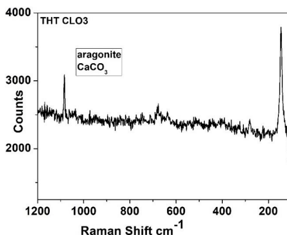
Figure 9. Raman spectrum of aragonite (CaCO 3 ) on coin THT CLO3.
