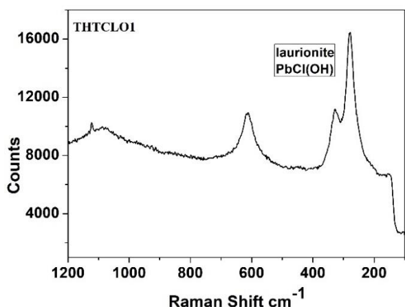
Figure 8. Raman spectrum of laurionite [PbCl(OH)] on coin THT CLO1.
