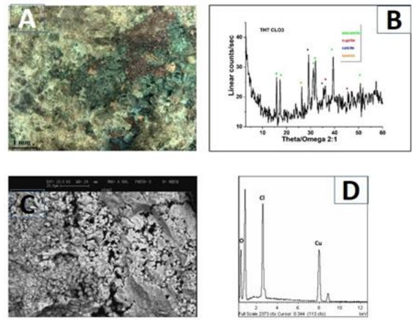
Figure 5. Coin THT CLO3: OM image (A), XRD spectrum (B), SEM image (C) and EDS spectrum (D).
