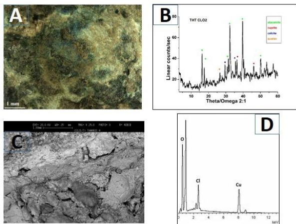
Figure 4. Coin THT CLO2: OM image (A), XRD spectrum (B), SEM image (C) and EDS spectrum (D).
