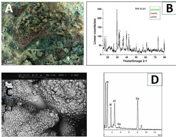
Figure 3. Coin THT CLO1: OM image (A), XRD spectrum (B), SEM image (C) and EDS spectrum (D).
