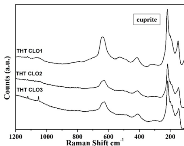
Figure 7. Raman spectra of cuprite (Cu 2 O) on the coins found at Tharros. The Raman spectra collected in a Cu-rich area evidence the presence of poorly crystallised cuprite.
