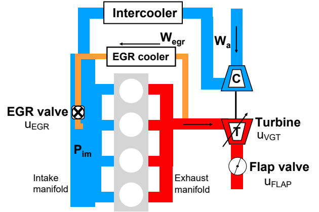
Fig. 1. FPT F1C Engine layout.
