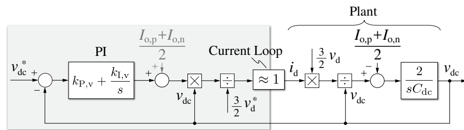
Figure 8. Detailed equivalent block diagram of the v_{dc} voltage control loop.
