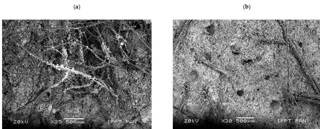
Figure 9. Microphotograph of the analysed fresh split surface of gypsum-based composites: (a) with sheep wool fibres and (b) with hemp fibres (scanning electron microscope, scale bar = 500 μm).
