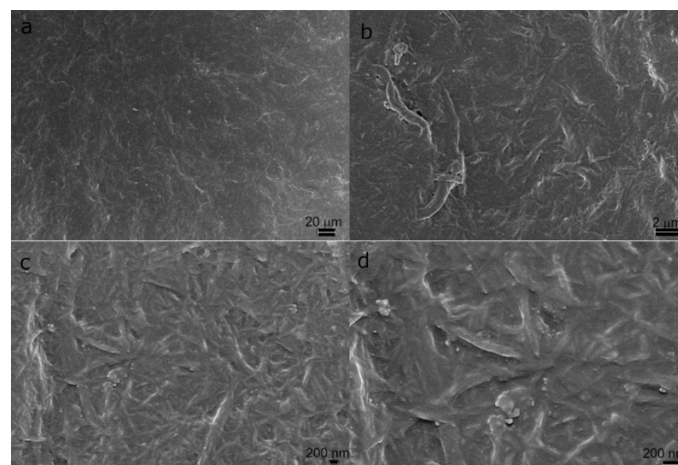
Figure 5. FE-SEM images of the surface of a composite with 15 wt% PI, irradiated for 5 min on each side, at increasing magnification: (a) shows a good macroscopic homogeneity of the surface; in (b) larger fibers, and pores in their vicinity, are visible; (c,d) show closer views of the surface of the composites evidencing the structure formed by the cellulose fibrils.
