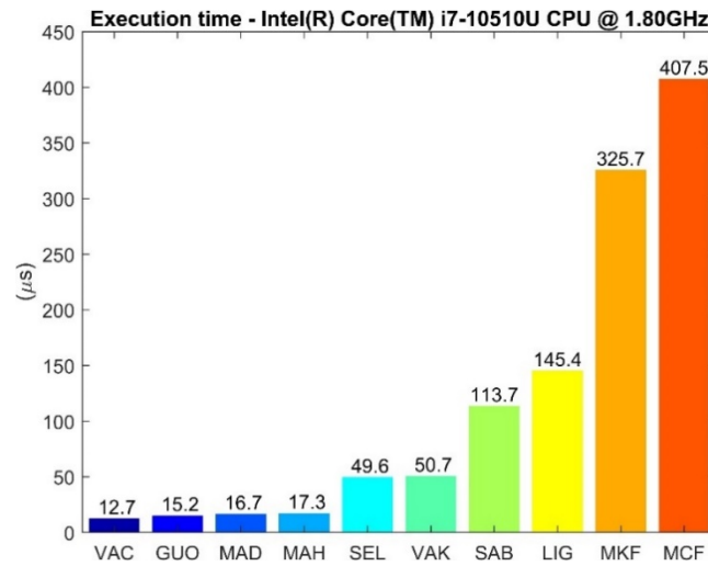
Figure 5. Execution time needed for a single update step by each SFA.
