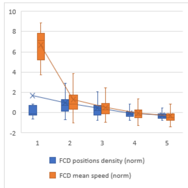
Figure 2 – Normalised FCD values for density and mean speed (Y axes) plotted against BDTRE functional classes (X axes).
