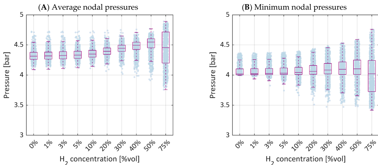
Figure 9. Evolution of average (A) and minimum (B) nodal pressures recorded in 1000 networks with increasing H 2 concentrations—pure H 2 injected within the network.
